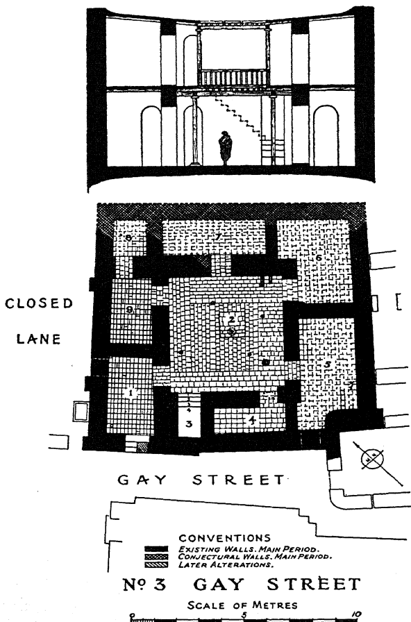
26. PLAN AND RECONSTRUCTION OF A PRIVATE HOUSE AT UR, OF THE PERIOD OF THE ISIN AND LARSA DYNASTIES
